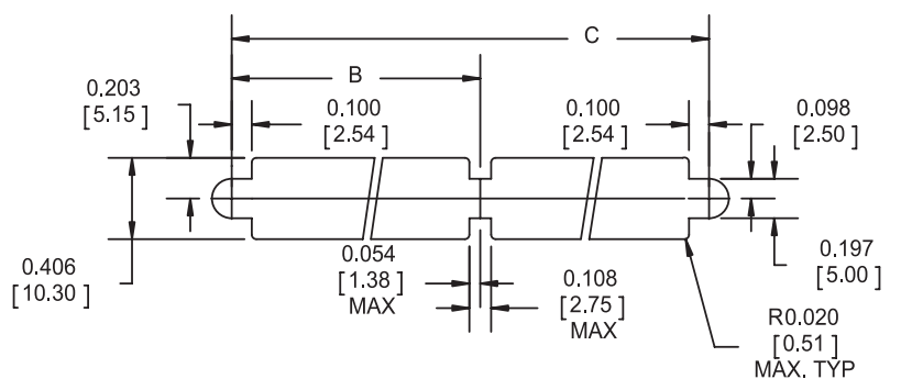
Float mounting Styles 13 & 23
