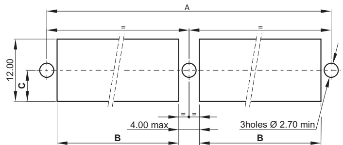
108 to 160 contacts
